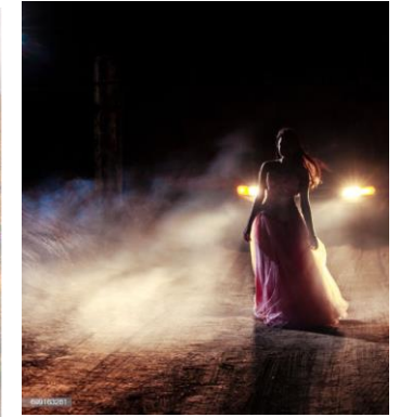
Ethereal
